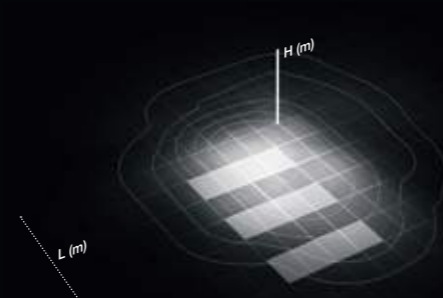
AP-D2 Pedestrian Crossing
