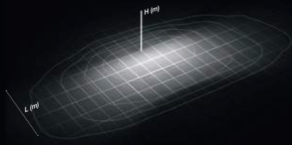
LA-03 Wide Street L / H = 1,25
