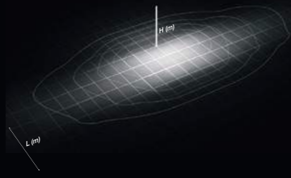
ST-02 Narrow Street L / H = 0,75
