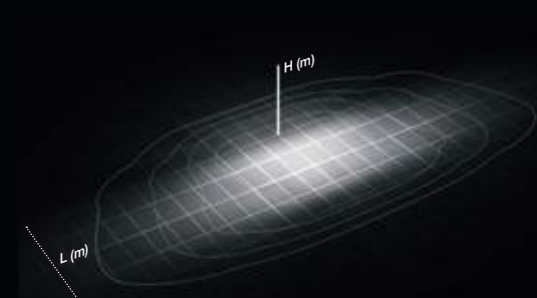
ME-05 Medium Street L / H = 1
