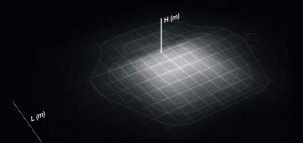
LT-64 Asymmetric Beam with backlight L/H = 2
